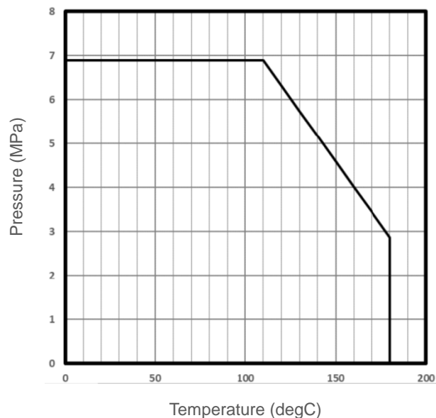
Fig. 1 Pressure – Temperature rating
